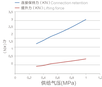
QQC-020S连接力、提升力曲线图 QQC-020S Continuous relay, lifting force curve
