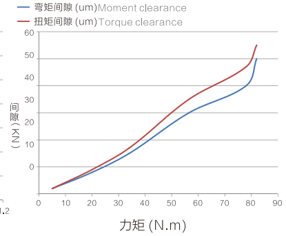
QQC-020S弯矩、扭矩变位曲线图 QQC-020S Bending moment and torque changer curve
