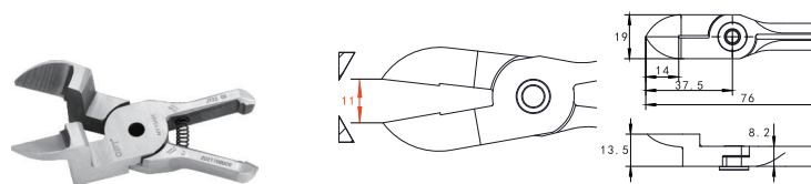
L形平嘴鉗 Crank blade
