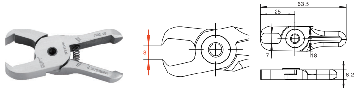
頂切平嘴鉗 Nipping blade
