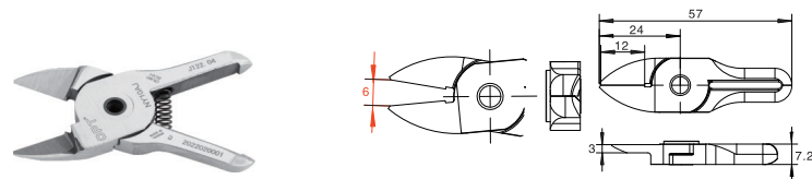
頂切平嘴鉗 Nipping blade
