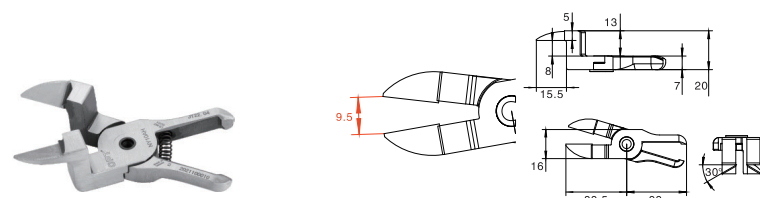
L形平嘴鉗 Crank blade
