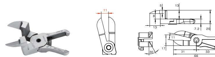
L形平嘴鉗 Crank blade
