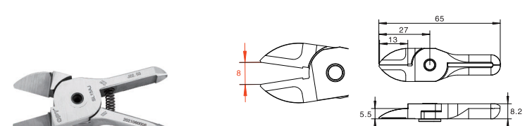
圓頭平嘴鉗 Straight blade
