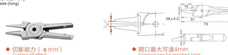
金屬尖頭平嘴鉗(加長) sharp straight blade (long)
