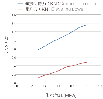
QQT-10 continuous relay and lifting force curve
