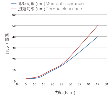
QQT-10 Bending moment and torque changer curve
