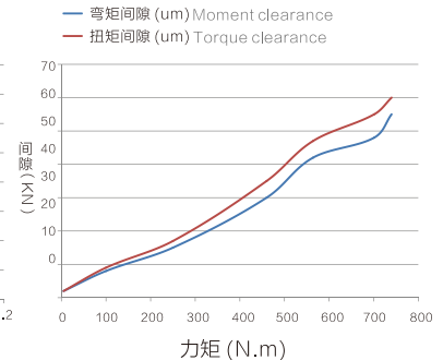
OQC-076弯矩、扭矩变位曲线图 OQC-076Bending moment and torque changer curve
