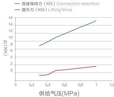
OQC-076连接力、提升力曲线图 OQC-076 Continuous relay, lifting force curve
