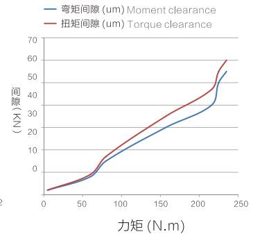
OQC-040弯矩、扭矩变位曲线图 OQC-040 Bending moment and torque changer curve
