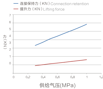
OQC-040连接力、提升力曲线图 OQC-040 Continuous relay, lifting force curve
