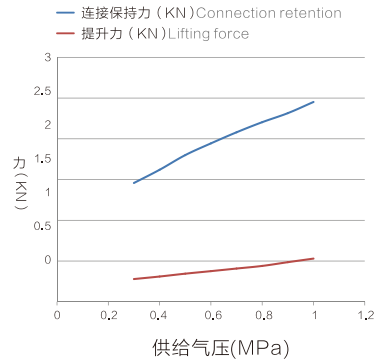
OQC-015连续继电器、提升力曲线图 OQC-015 Continuous relay, lifting force curve
