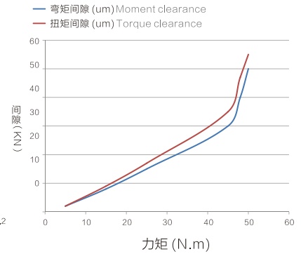
OQC-015弯矩、扭矩变位曲线图 OQC-015 Bending moment and torque changer curve
